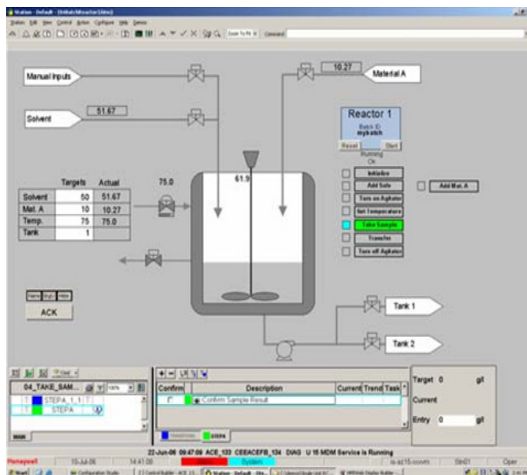
Typical Batch Manager Display
