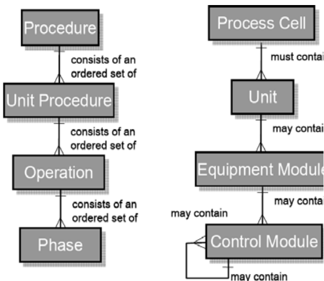
Overview of ISA S88.01
