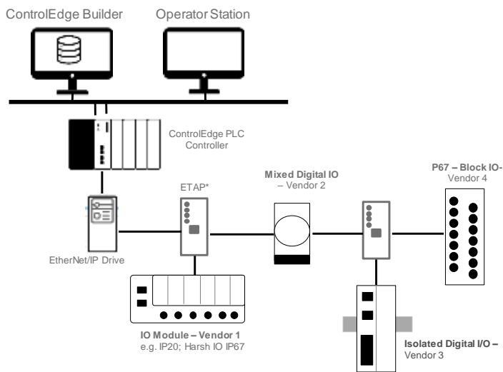
Figure 7 – Multivendor EtherNet/IP device and I/O module connectivity
