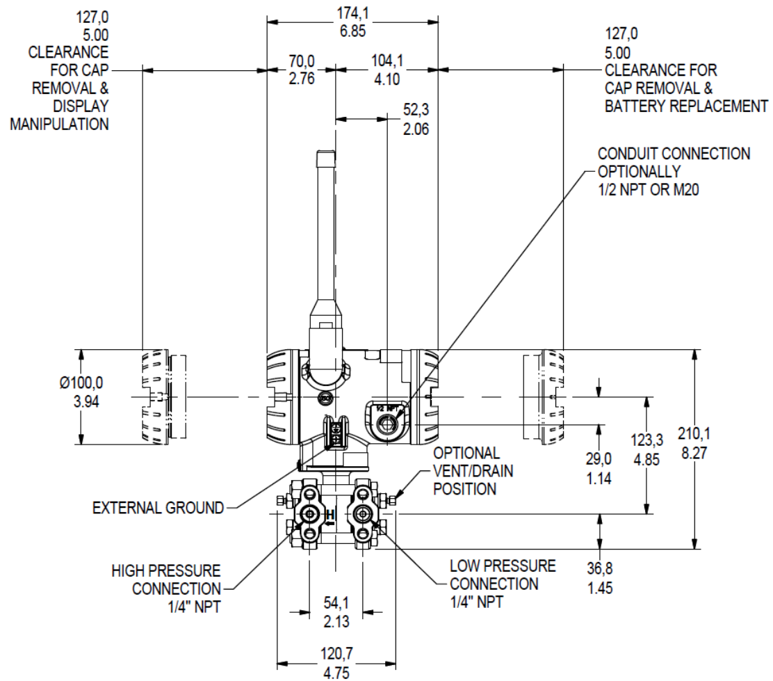
Figure 4-1 Dimensions of a typical SmartLine Wireless Transmitter with the 4 dBi Integral Antenna Option
