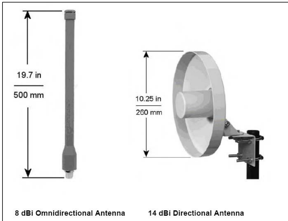
Figure 6-1 Remote Antennas
