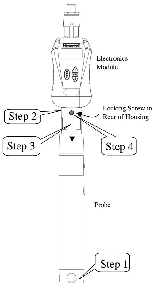
Figure 2-3 Integral Mounting
