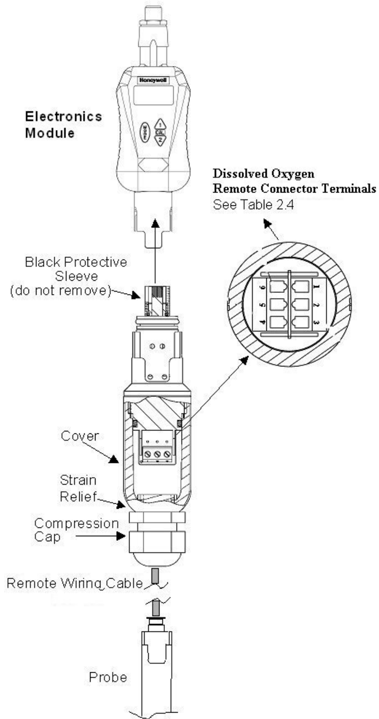
Remote Electronics for Module DL5000 Dissolved Oxygen Probes
